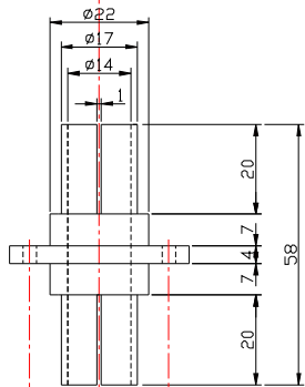
Priruba posuvu Material: MS
