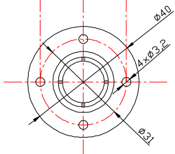
Priruba posuvu Material: MS
